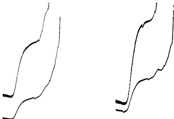
Fig. 1.—Reduction waves of phytol chain in chlorophylls: 1 ml. of dioxane solution of the chlorophylls added to 10 ml. of 0.1 molar tetramethylammonium bromide. Camera opened at 1.60 volts applied cathodic potential. Upper curves at sensitivity 20, lower curves at sensitivity 50 of Sargent Polarograph. Chlorophyll a on left, chlorophyll b on right half of figure. Diffusion currents: 3.0 microamperes for chlorophyll a, 5.1 microamperes for chlorophyll b. Approximate concentrations of dioxane extracts: 3.3 millimoles per liter for chlorophyll a, 5.6 millimoles per liter for chlorophyll b.
